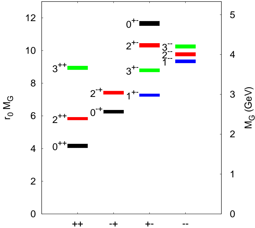
Figure 4: (color online) The mass spectrum of glueballs. The height of each box indicates the statistical uncertainty. Figure used with permission from reference [35].
