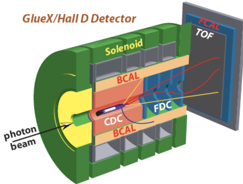
Figure 26: Layout of the GlueX Experiment at Jefferson Laboratory
