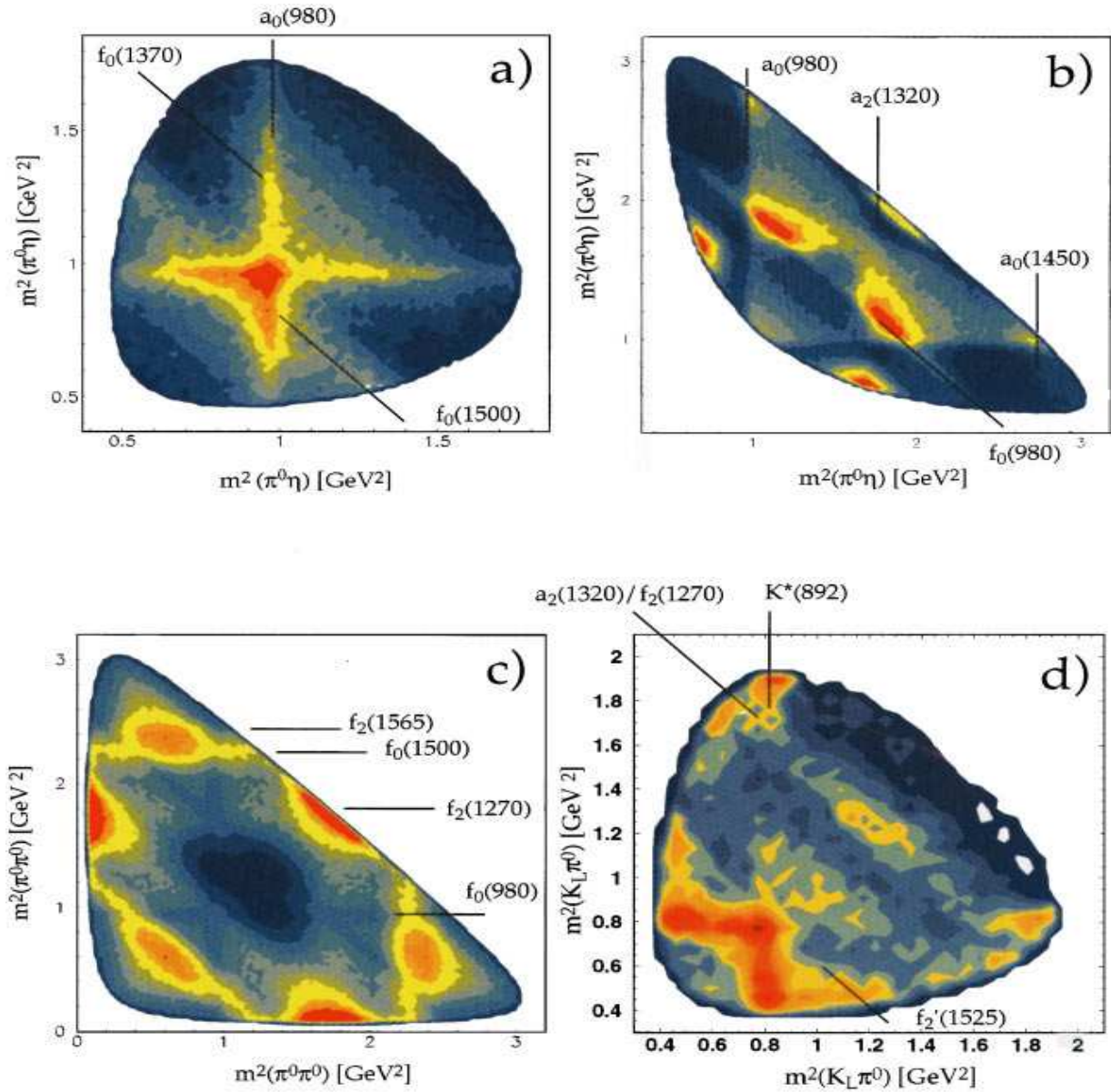
Figure 10: Dalitz plots for p\bar{p} annihilation at rest from Crystal Barrel into (a) \pi^0\eta\eta ( \sim 2 \times 10^5 events), (b) \pi^0\pi^0\eta ( \sim 2.8 \times 10^5 events), (c) 3\pi^0 ( \sim 700,000 events), (d) \pi^0 K_L K_L ( \sim 37,000 events). All events are entered more than once for symmetry reasons. Figure taken from [2].
