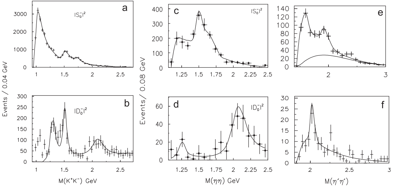
Figure 14: K^+K^- S - (a) and D -wave (b) from a coupled-channel analysis of WA102 \pi^+\pi^- and K^+K^- data [133]. The T-matrix formalism was used for overlapping resonances to account for unitarity. Signals for f_0(1500) and f_0(1710) are clearly observed. Mass distributions for \eta\eta S - and D -wave are shown in (c) and (d). The right panels show \eta\eta' (e) and \eta'\eta' (f) mass distributions.
