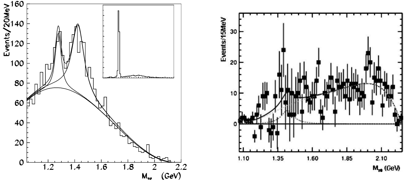
Figure 20: Invariant \gamma V mass distributions for V = \rho (left) and V = \phi (right) from [100]. The insert shows the full mass scale with the \eta' clearly visible. The \gamma\phi distribution is side-band background subtracted and no structure is observed around 1400 \text{MeV}/c^2 .
