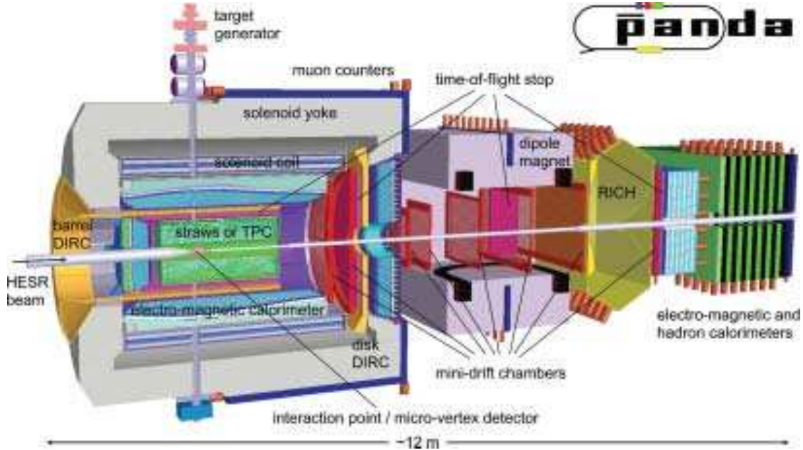
Figure 27: Layout of the PANDA experiment at GSI: antiprotons from the HESR enter from the left and hit clusters or pellets of hydrogen at the interaction point, which is surrounded by detectors inside a solenoid magnet.
