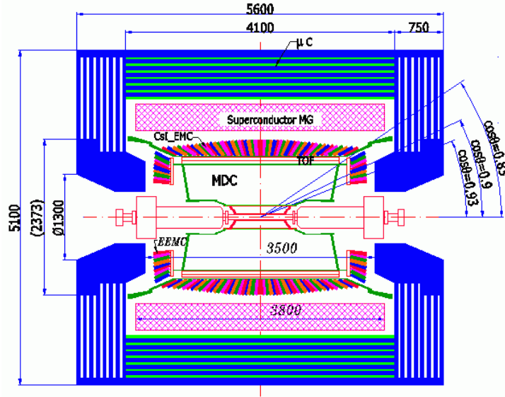
Figure 25: Layout of the BES-III Experiment at BEPCII [88].
