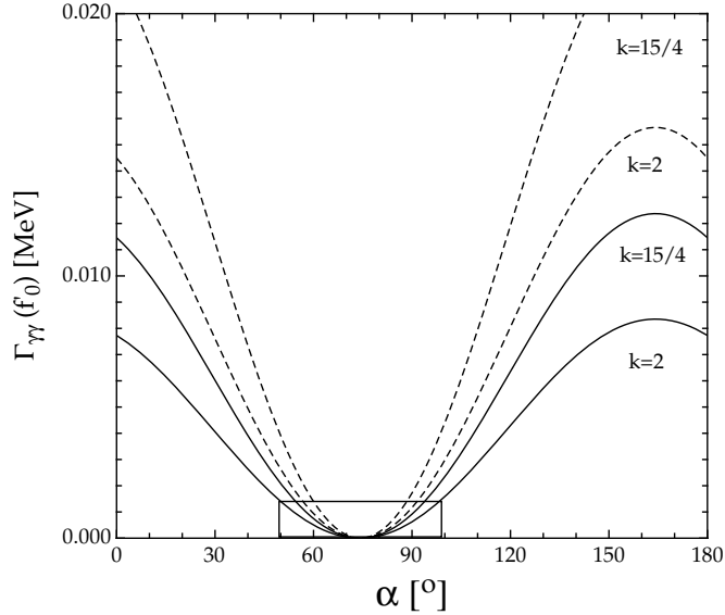
Figure 24: Predicted two-photon width for the f_0(1500) (solid curves) and f_0(1710) (dashed curves) assuming a q\bar{q} structure. The box shows the 95% confidence-level upper limit from ALEPH for the f_0(1500) . The picture is taken from [184].
