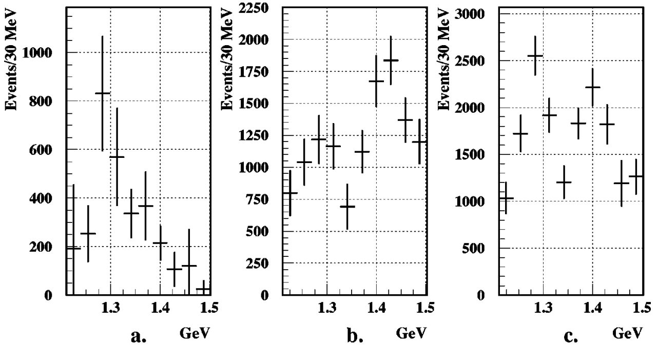
Figure 22: Fitted intensity distributions from E852 for the 0^{-+} wave [206]: (a) a_0\pi intensity, (b) \eta(\pi\pi)_S intensity, and (c) total 0^{-+} intensity. A sharp peak at about 1300 MeV/ c^2 is visible in (a), consistent with the assumption of \eta(1295) \rightarrow a_0(980)\pi .
