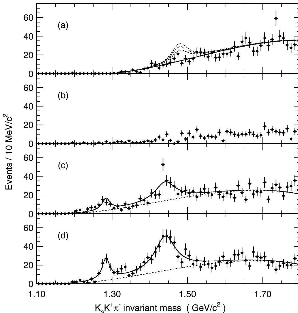
Figure 19: Distributions of the K_S^0 K^\pm \pi^\mp invariant mass from CLEO for data events detected with (a) p_\perp \leq 100 MeV/ c , (b) 100 MeV/ c \leq p_\perp \leq 200 MeV/ c , and (c) 200 MeV/ c \leq p_\perp \leq 600 MeV/ c in the untagged mode, and (d) for all p_\perp in the tagged mode [143]. The dashed curves in (a) show the strength of the expected \eta(1475) signal according to the L3 results [148]. The solid curves in (a), (c) and (d) are the results of binned maximum likelihood fits for resonances with a polynomial approximation to the non-interfering combinatorial background. See text for details.
