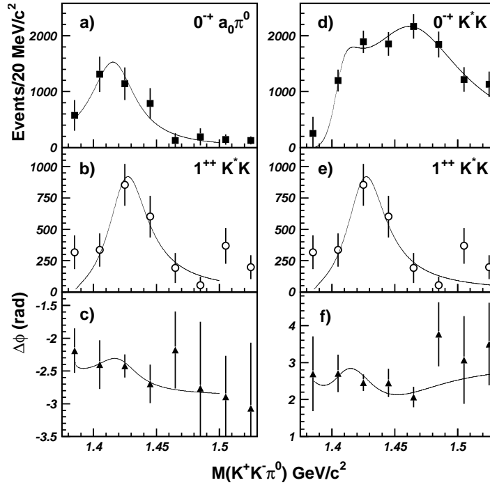
Figure 23: The intensity observed in the K\bar{K}\pi final state from E852 [207]. (a) shows the 0^{-+} intensity in the a_0(980)\pi partial wave, (b) and (e) show the 1^{++} intensity in the K^*K partial wave, (d) shows the 0^{-+} intensity in the K^*K partial wave, and (c) and (f) shows the phase differences between (a) and (b) and between (d) and (e) respectively.
