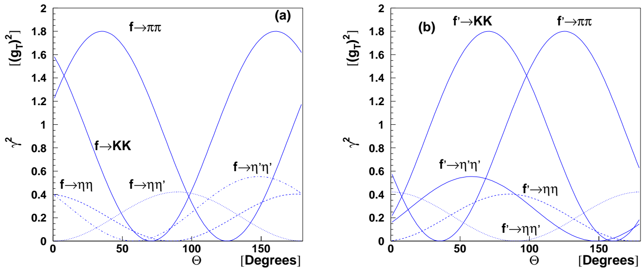
Figure 2: The decay amplitude, \gamma^2 , as a function of the nonet mixing angle, \theta . (a) is for f decays while (b) is for f' decays. In this particular example, the pseudoscalar mixing angle is taken as \theta_P = -17^\circ .
