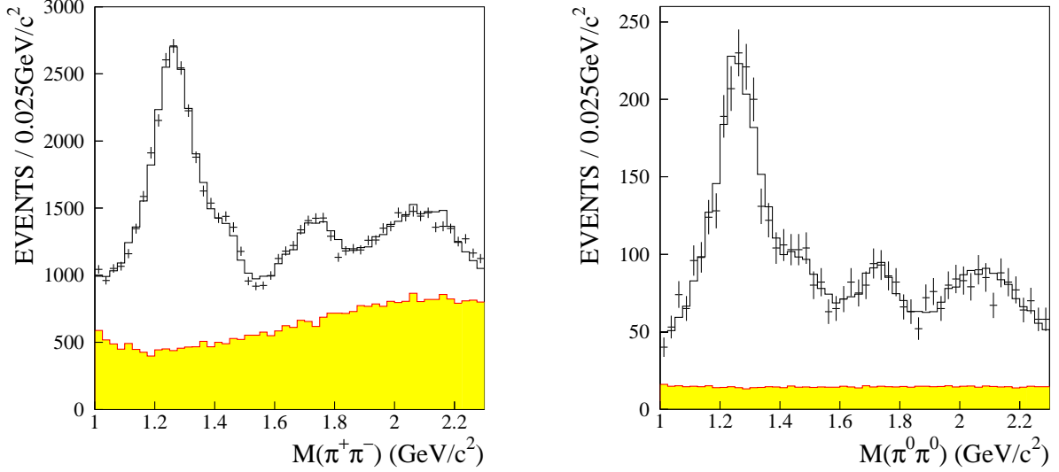
Figure 15: The \pi^+\pi^- invariant mass distribution (a) and the \pi^0\pi^0 mass distribution (b) from the reaction J/\psi \rightarrow \gamma\pi\pi from BES [102]. The crosses are data, the full histogram shows the maximum likelihood fit, and the shaded area corresponds to the background.
