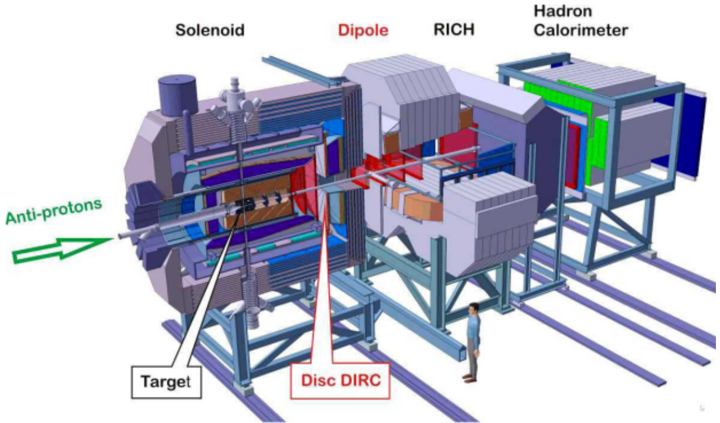
Figure 27: Layout of the PANDA experiment at GSI: antiprotons from the HESR enter from the left and hit clusters or pellets of hydrogen at the interaction point, which is surrounded by detectors inside a solenoid magnet.
