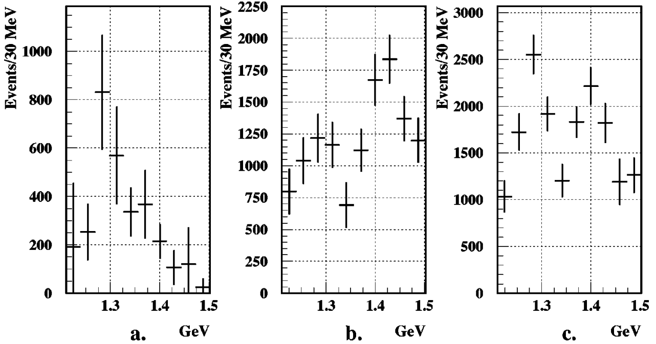
Figure 22: Fitted intensity distributions from E852 for the 0^{-+} wave [211]: (a) a_0\pi intensity, (b) \eta(\pi\pi)_S intensity, and (c) total 0^{-+} intensity. A sharp peak at about 1300 \text{MeV}/c^2 is visible in (a), consistent with the assumption of \eta(1295) \rightarrow a_0(980)\pi .
