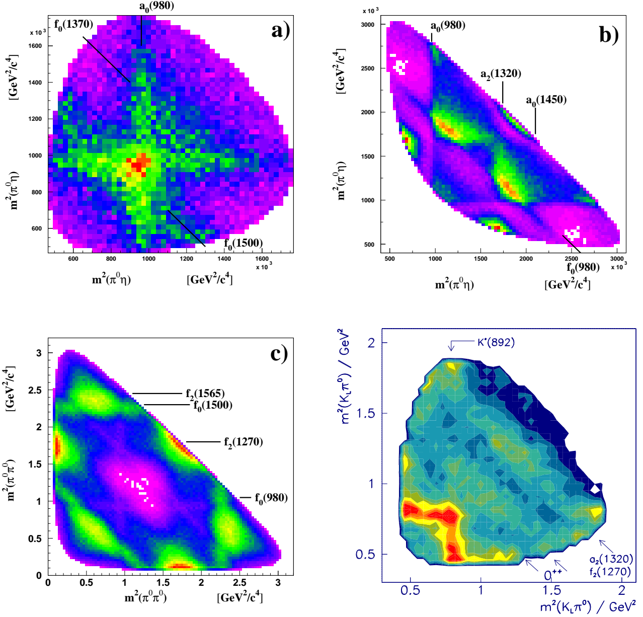
Figure 10: Dalitz plots for p\bar{p} annihilation at rest from Crystal Barrel into (a) \pi^0\eta\eta ( \sim 2 \times 10^5 events), (b) \pi^0\pi^0\eta ( \sim 2.8 \times 10^5 events), (c) 3\pi^0 ( \sim 700,000 events), (d) \pi^0 K_L K_L ( \sim 37,000 events). All events are entered more than once for symmetry reasons. Figure taken from [2].
