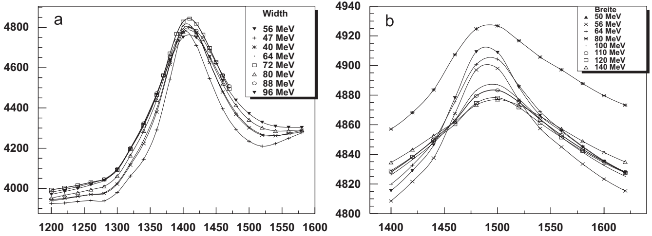
Figure 12: Analysis of the annihilation reaction p\bar{p} \rightarrow \pi^+\pi^-\pi^+\pi^-\eta [175]: mass scans for I^G J^P = 0^+ 0^\pm resonances assuming different widths. (a) The left side shows a clear peak identified as the \eta(1405) . (b) The right side shows the search for a second pseudoscalar state indicating the presence of the \eta(1475) with (M = 1490 \pm 15, \Gamma = 74 \pm 10) \text{ MeV}/c^2 .
