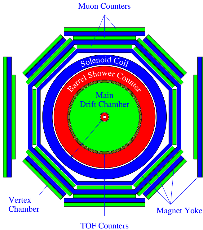
Figure 7: End view of the BES-II detector at IHEP, Beijing [6, 93].
