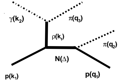
Fig. 3. The t-channel exchange diagram for double meson photoproduction reactions
