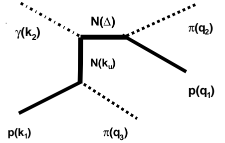
Fig. 5. A u-channel exchange diagram for production of a baryon resonance in photoproduction of two mesons
