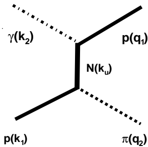
Fig. 4. The u-channel exchange diagram for photoproduction of single mesons
